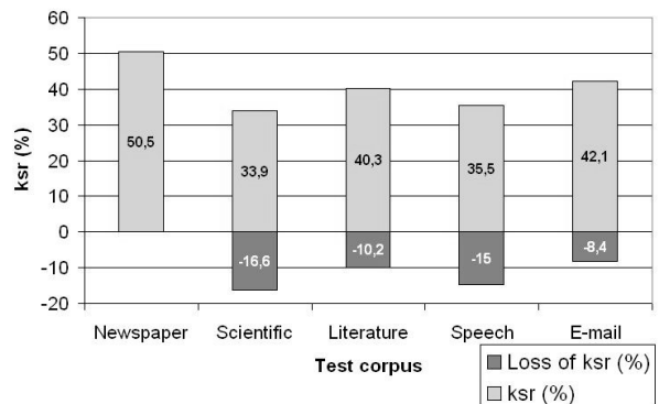
Figure 2: Results ( ksr ) for the five test corpora
